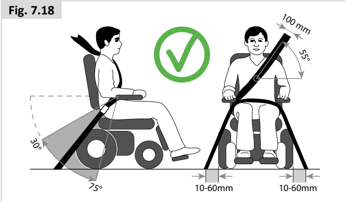
For use with Dahl Docking system only (Fig. 7.18) When using wheelchair with Dahl Docking system, the floor anchorage points for occupant restraint should be located 10-60 mm outside wheels, on each side.
